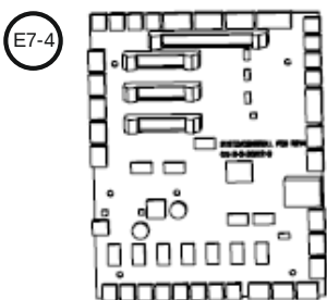
PCB Sysco REV4 E/S+/SP4 05-3-3-3002-1
